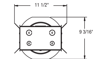
(Ceiling Opening = 6 3/4")
