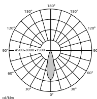
Stralingshoek 27°
