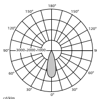
Stralingshoek 40°
