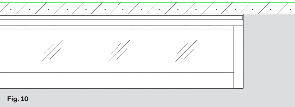
Wall mounting with a full-length wall profile The wall profile can be designed to match the length of the luminaire, creating a cohesive visual unit while also providing additional space for accessory mounting.
