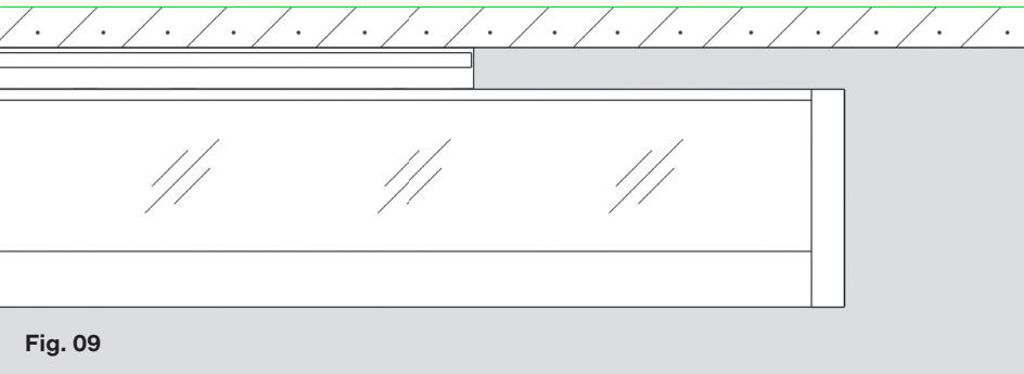
Wall mounting with a short wall profile The wall profile enhances the visual lightness of the luminaire. Additionally, it offers an option for accessory installation.
