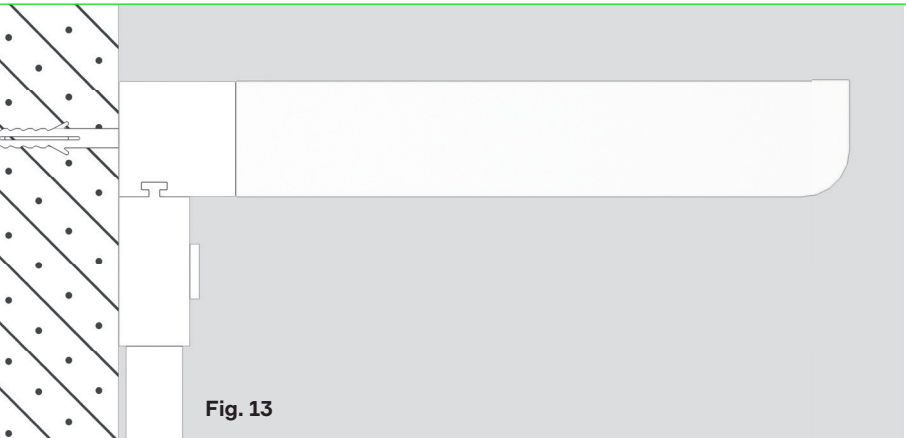
Wall mounting with wall profile The wall channel provides the option to accommodate various accessory components.
