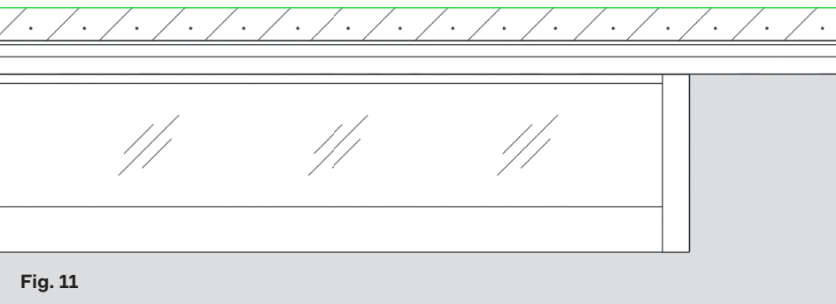
Wall mounting with a continuous wall profile The continuous wall profile can be used as a cable channel during a subsequent installation. It also allows for flexible positioning within the room.
