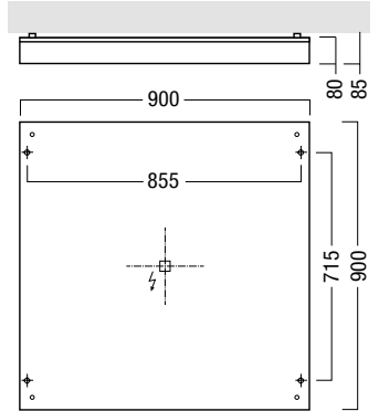
CIELOS 1C 900 T16
