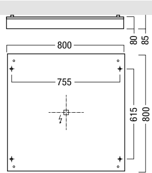
CIELOS 1C 800 LED
