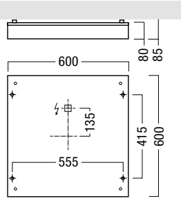
CIELOS 1C 600 T16/LED
